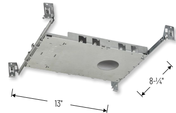
NHIOFK-1 New Construction Frame-In for 1" Remodel Housing
